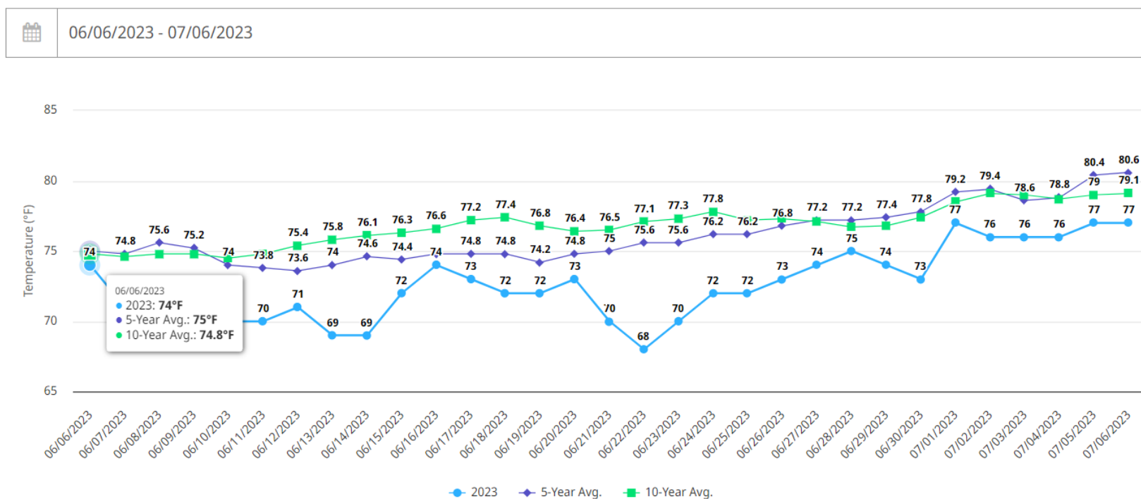
Average Soil Temperature in Loudon, TN (37774)
